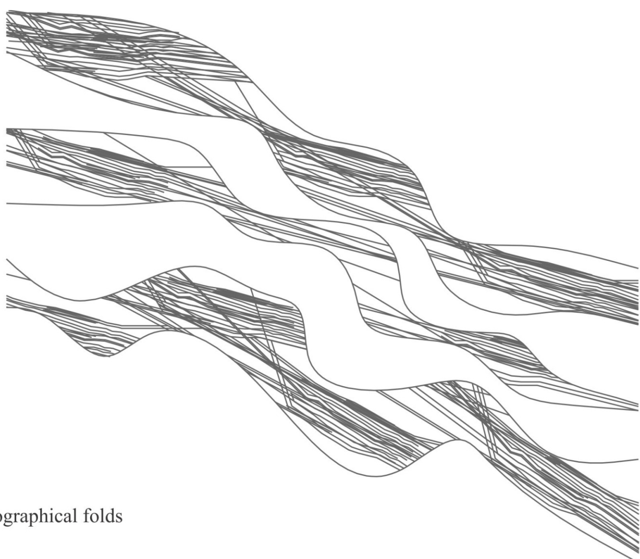
topographical folds
